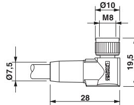
Dimensional drawing
